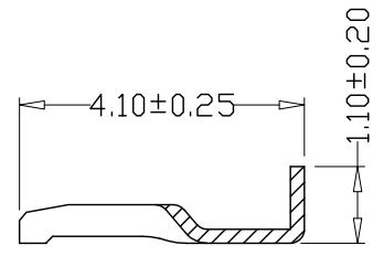
SEC:C-C
